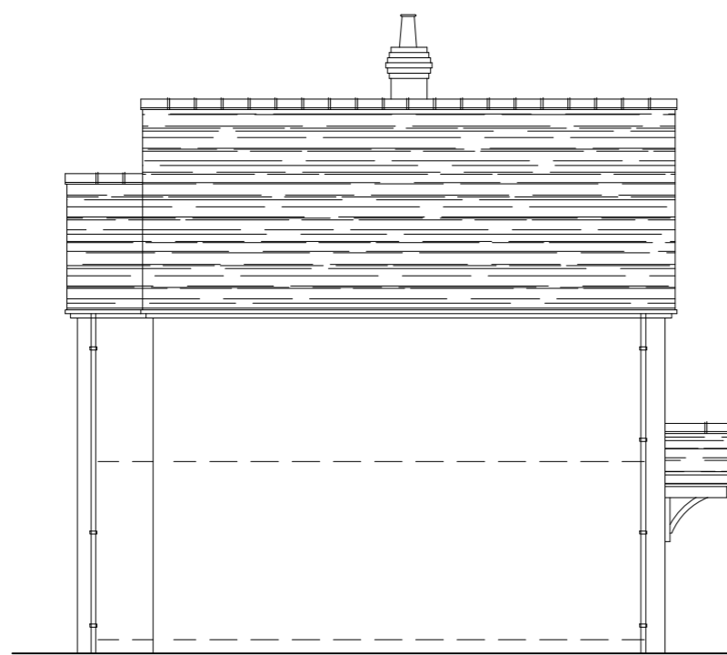
North West Elevation
