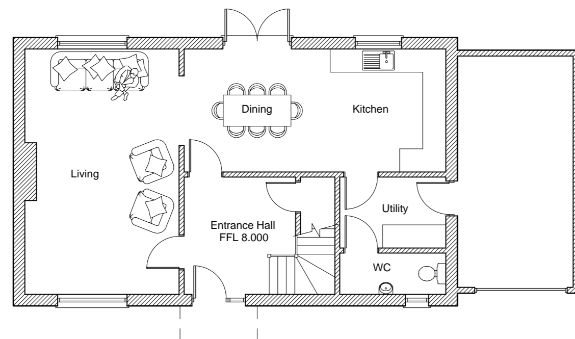
Ground Floor Plan Plot 1
