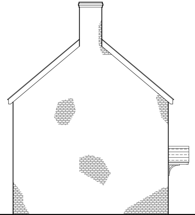
Plot 1 Southeast Elevation
