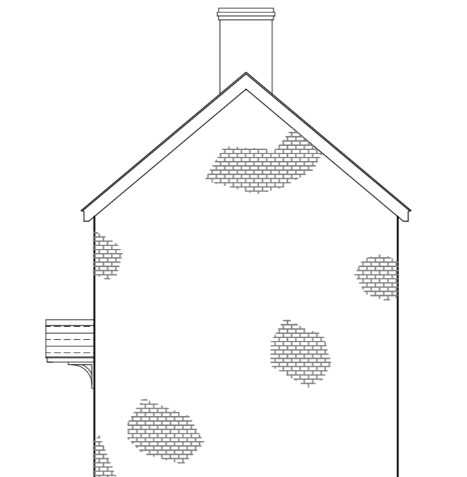
Plot 5 Southeast Elevation
