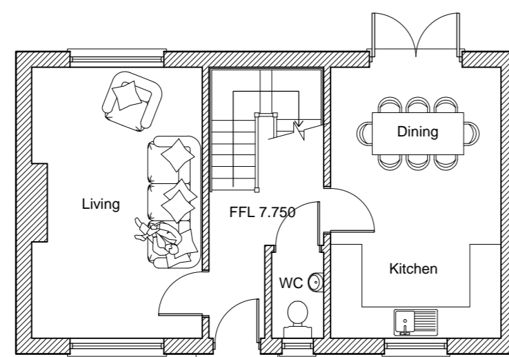
Ground Floor Plan Plot 5
